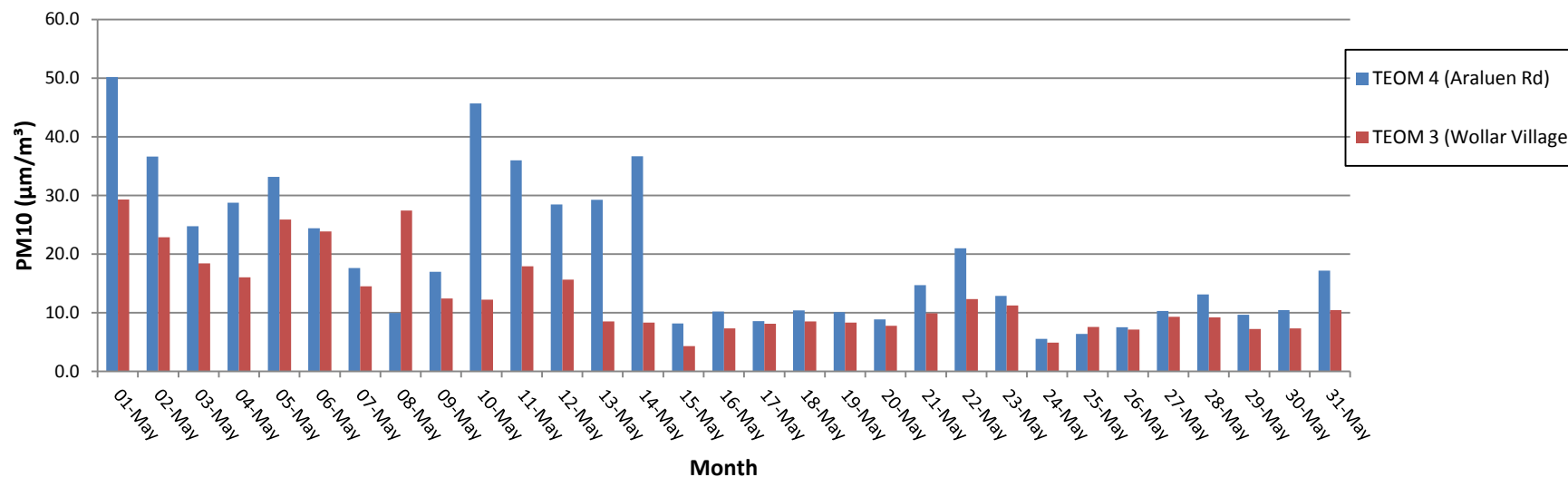
Figure 3. TEOM - 24 Hour Average PM10 Concentration ( \mu\text{g}/\text{m}^3 )
