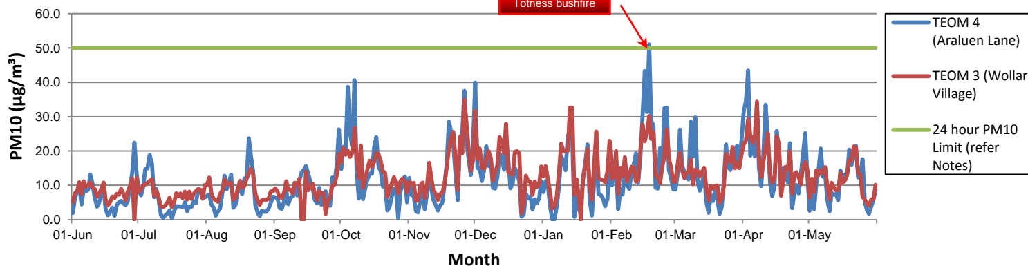
Figure 3. TEOM (PM10) Results - 12 Month Trend
