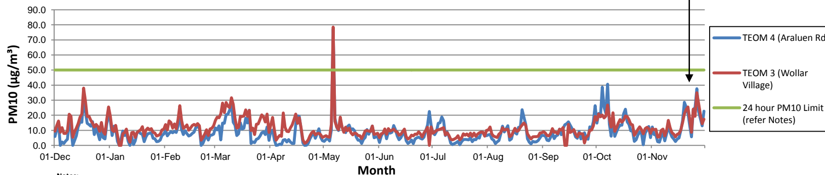
Figure 3. TEOM (PM10) Results - 12 Month Trend
