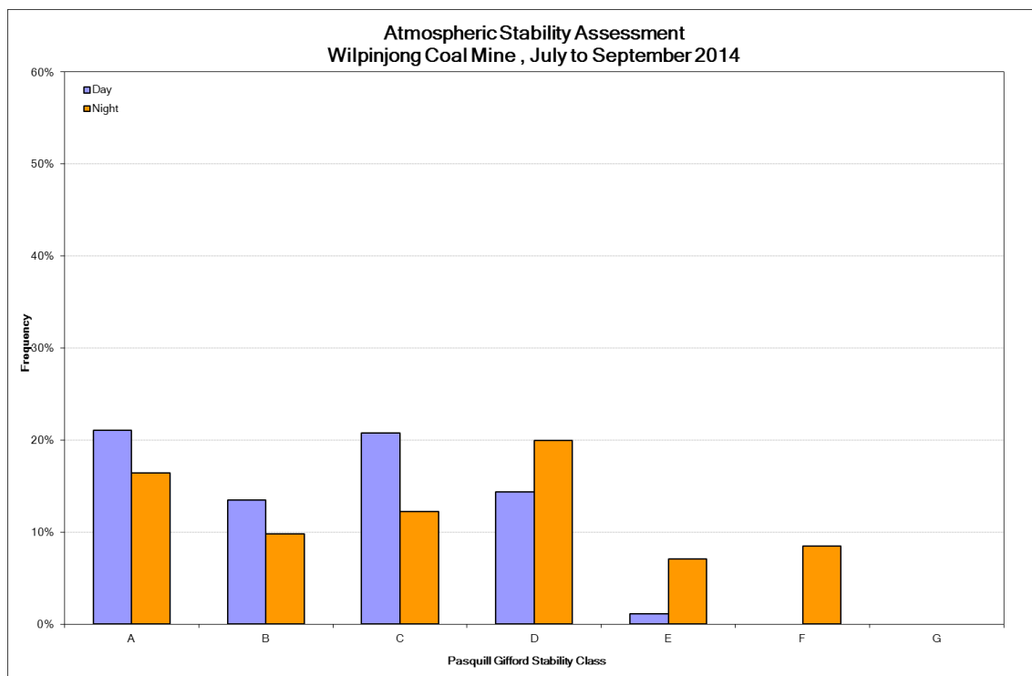
Figure 4: Assessment of temperature inversion frequency
