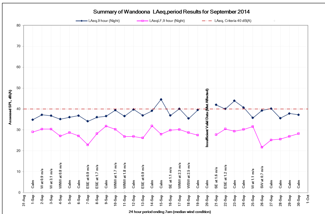
Figure 14: Night time noise levels at the Wandoona property, September 2014
