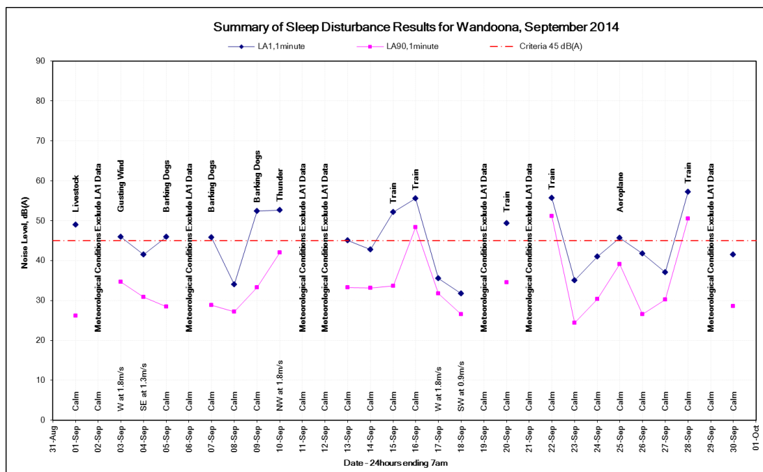
Figure 23: L_{A1,1\text{minute}} noise levels at the Wandoona monitoring location, September 2014
