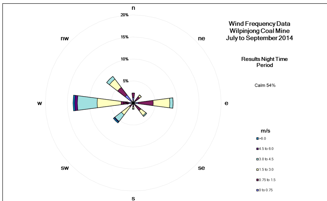
Figure 3: Wind rose for night period, all classes
