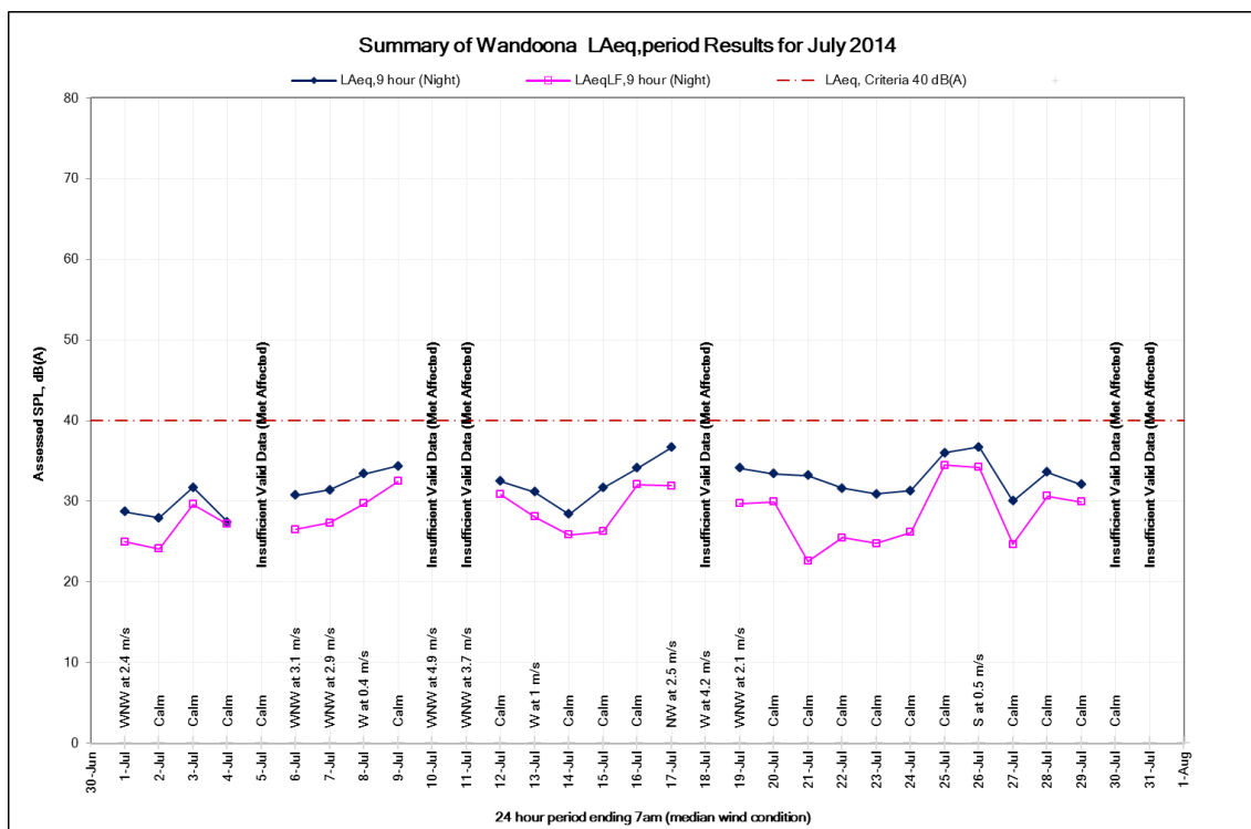
Figure 12: Night time noise levels at the Wandoona property, July 2014
