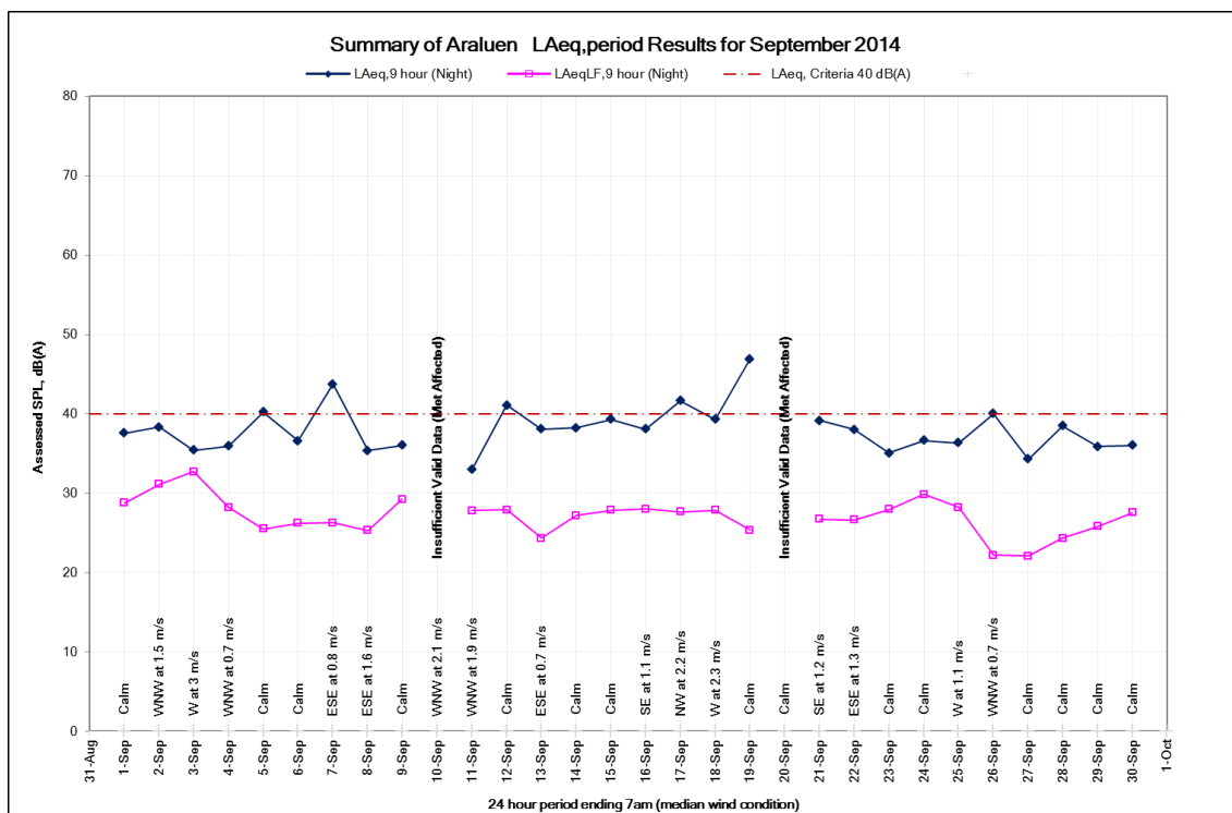
Figure 17: Night time noise levels at the Araluen monitoring location, September 2014
