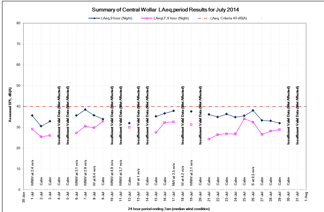
Figure 18: Night time noise levels at the Central Wollar monitoring location, July 2014
