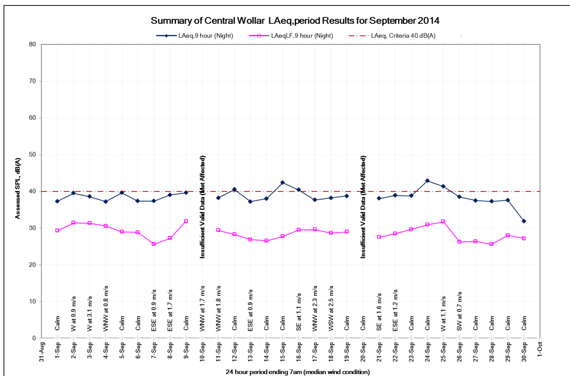
Figure 20: Night time noise levels at the Central Wollar monitoring location, September 2014
