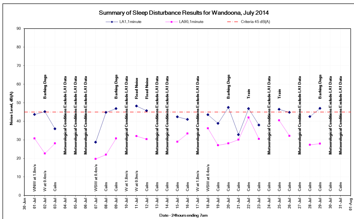
Figure 21: L_{A1,1\text{minute}} noise levels at the Wandoona monitoring location, July 2014
