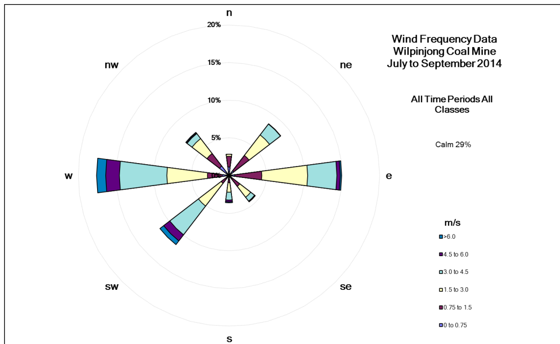
Figure 2: Wind rose for all periods, all classes
