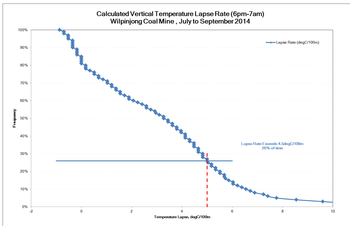
Figure 5: Temperature lapse rates, direct measurement analysis
