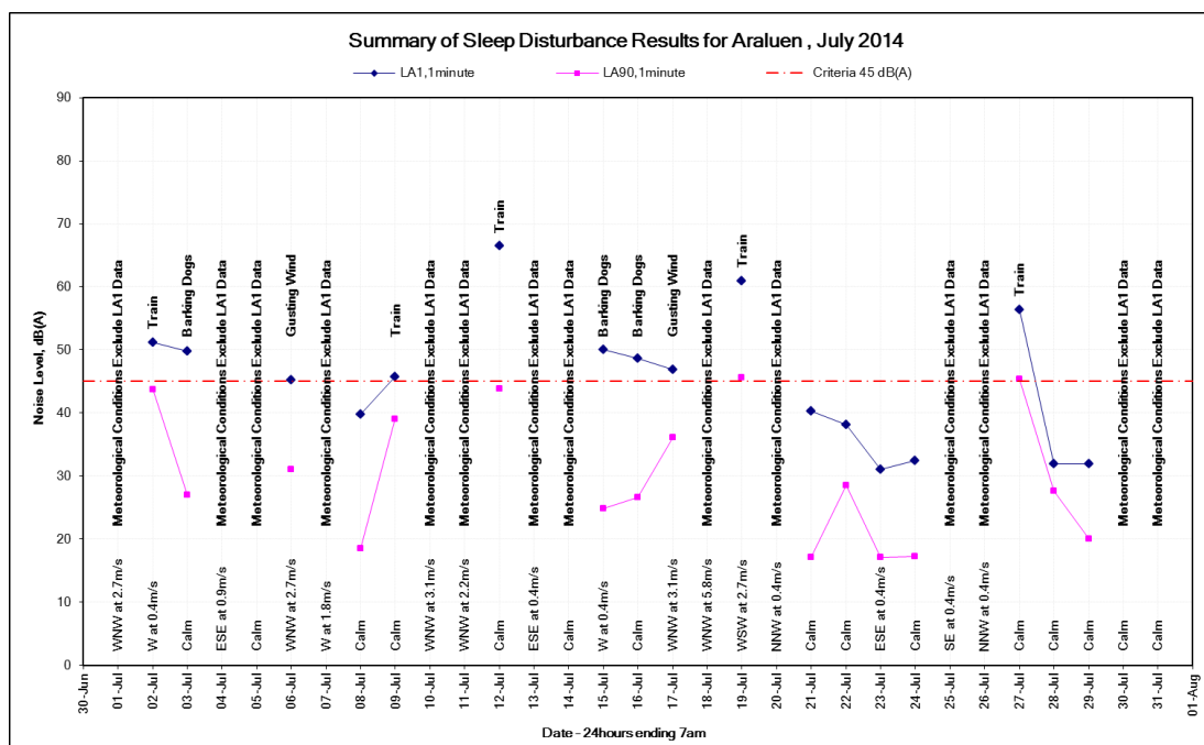
Figure 24: L_{A1,1\text{minute}} noise levels at the Araluen monitoring location, July 2014
