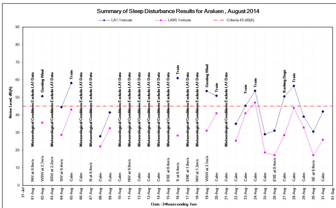
Figure 25: L_{A1,1\text{minute}} noise levels at the Araluen monitoring location, August 2014
