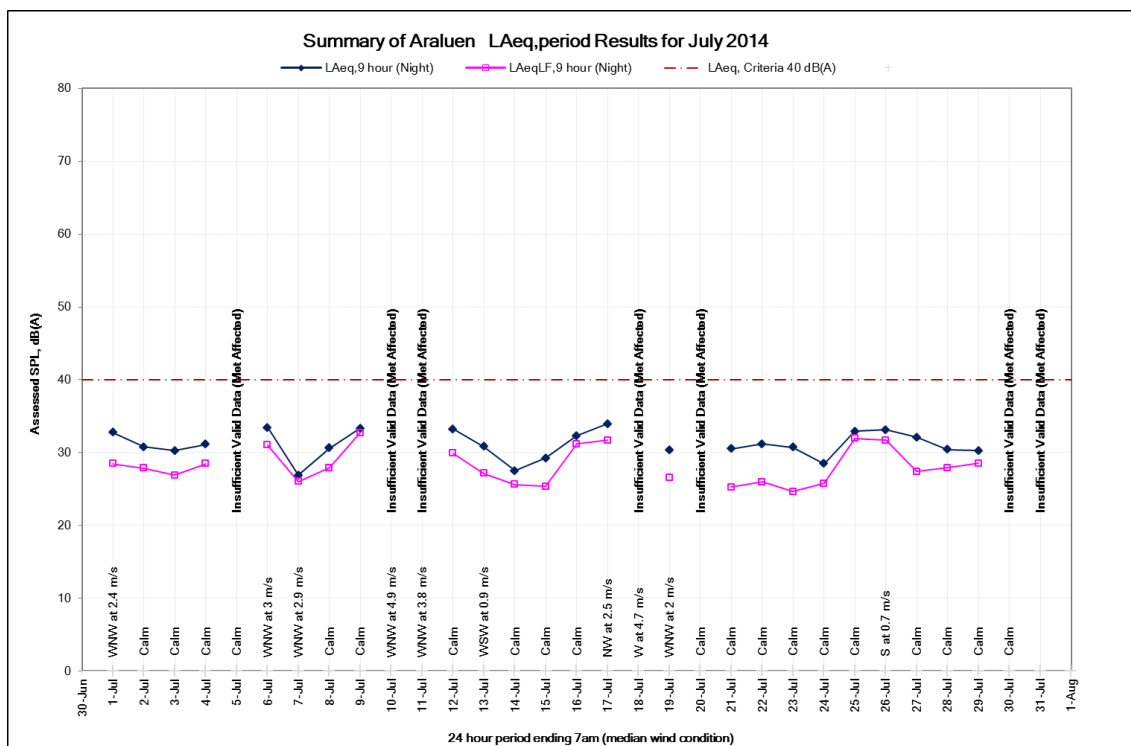
Figure 15: Night time noise levels at the Araluen monitoring location, July 2014
