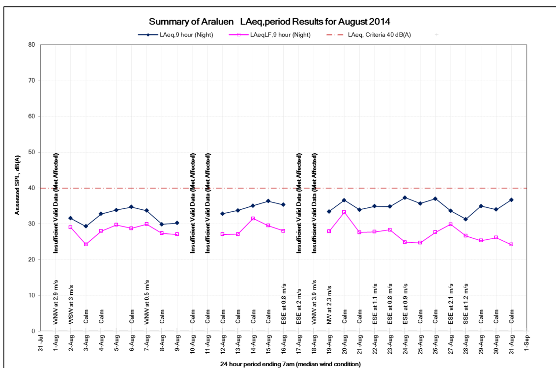
Figure 16: Night time noise levels at the Araluen monitoring location, August 2014
