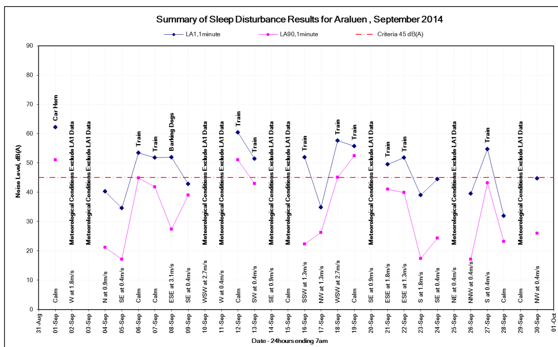
Figure 26: L_{A1,1\text{minute}} noise levels at the Araluen monitoring location, September 2014
