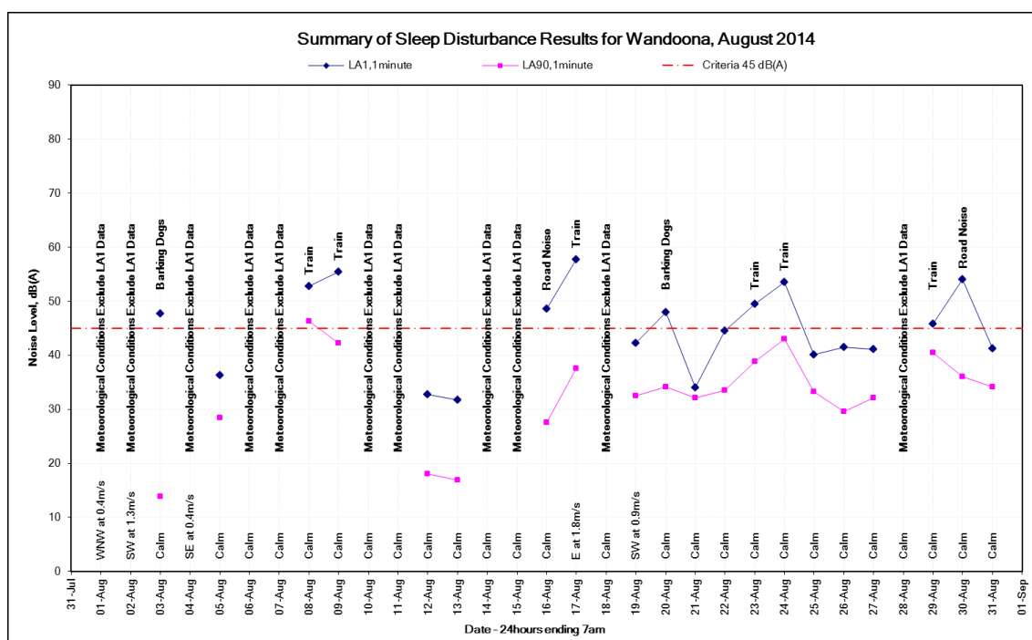
Figure 22: L_{A1,1\text{minute}} noise levels at the Wandoona monitoring location, August 2014
