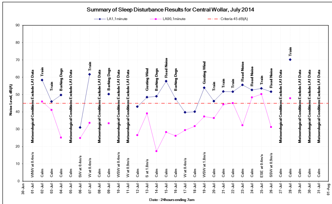
Figure 27: L_{A1,1\text{minute}} noise levels at the Central Wollar monitoring location, July 2014
