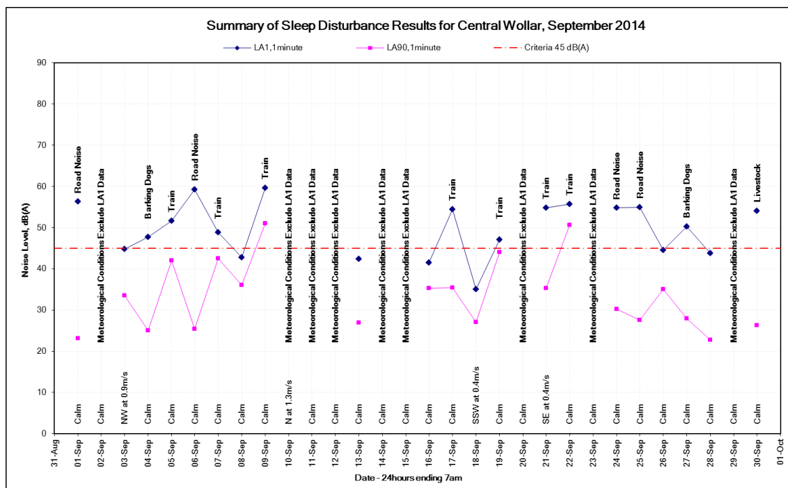
Figure 29: L_{A1,1\text{minute}} noise levels at the Central Wollar monitoring location, September 2014
