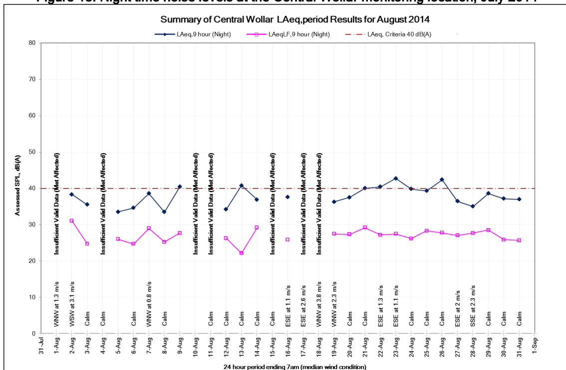
Figure 19: Night time noise levels at the Central Wollar monitoring location, August 2014
