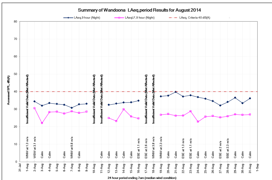
Figure 13: Night time noise levels at the Wandoona property, August 2014
