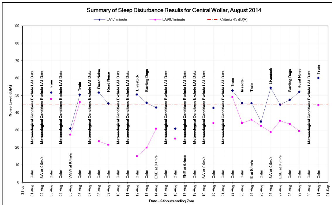
Figure 28: L_{A1,1\text{minute}} noise levels at the Central Wollar monitoring location, August 2014
