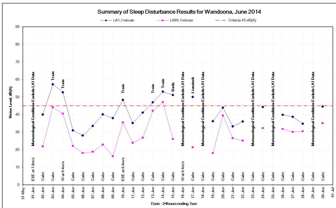
Figure 23: L A1,1minute noise levels at the Wandoona monitoring location, June 2014
