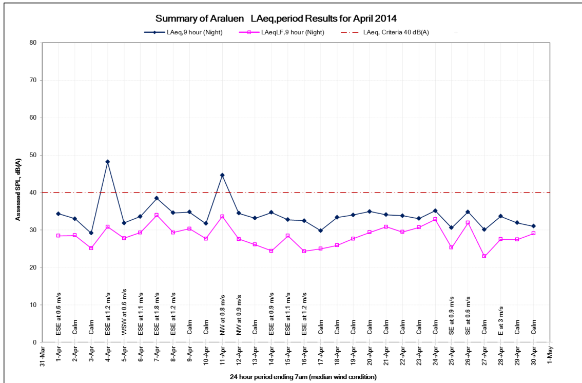
Figure 15: Night time noise levels at the Araluen monitoring location, April 2014
