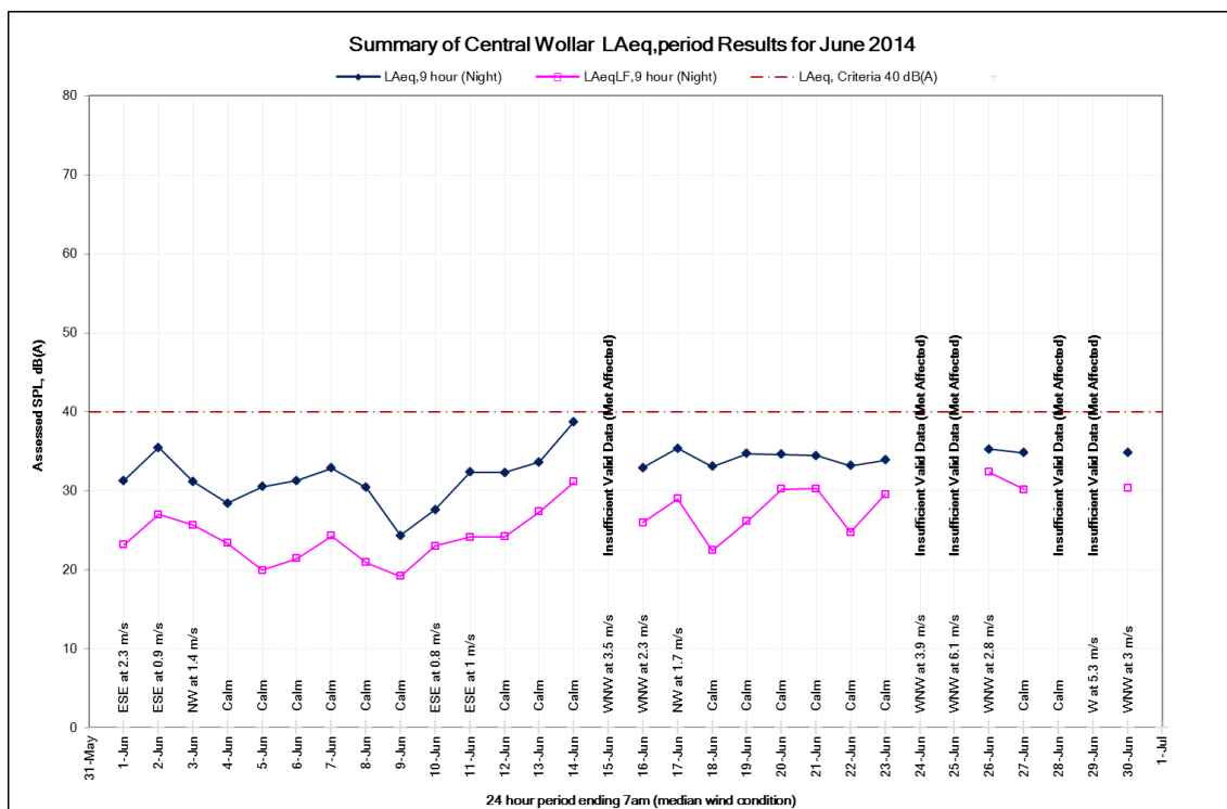
Figure 20: Night time noise levels at the Central Wollar monitoring location, June 2014
