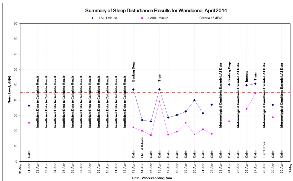
Figure 21: L_{A1,1\text{minute}} noise levels at the Wandoona monitoring location, April 2014
