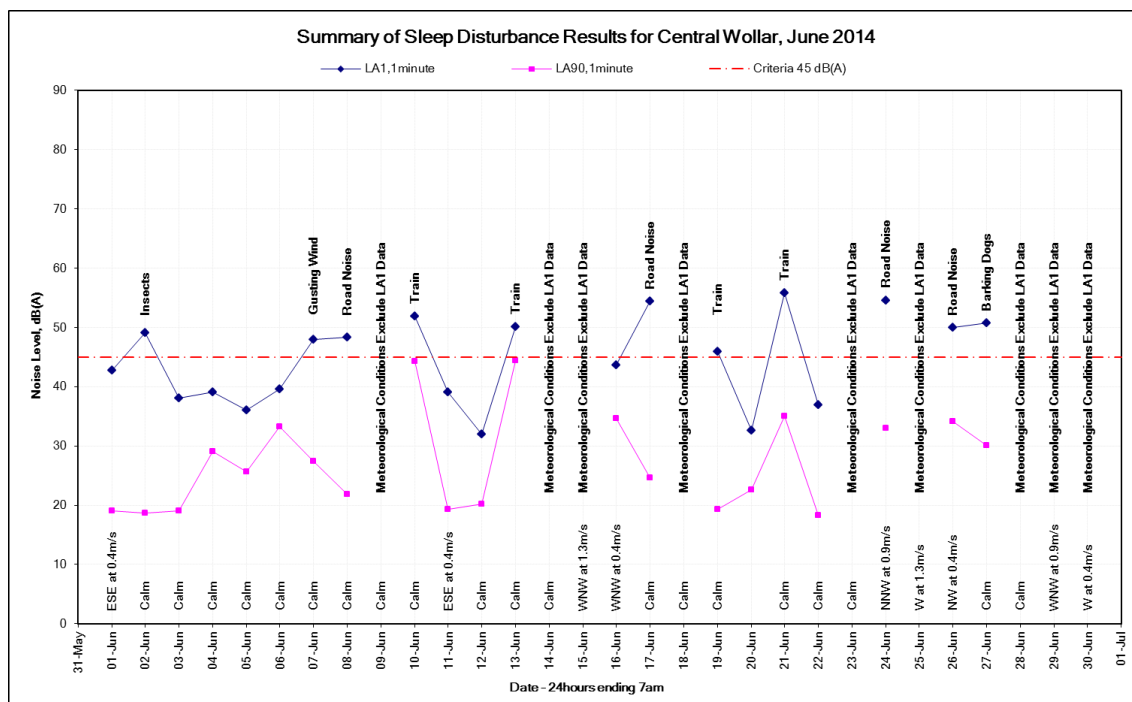
Figure 29: L_{A1,1\text{minute}} noise levels at the Central Wollar monitoring location, June 2014
