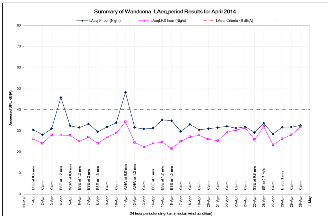
Figure 12: Night time noise levels at the Wandoona property, April 2014
