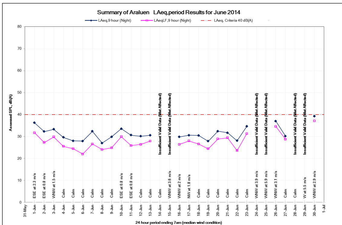
Figure 17: Night time noise levels at the Araluen monitoring location, June 2014
