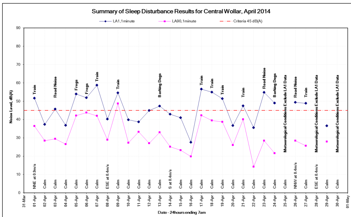
Figure 27: LA1,1minute noise levels at the Central Wollar monitoring location, April 2014
