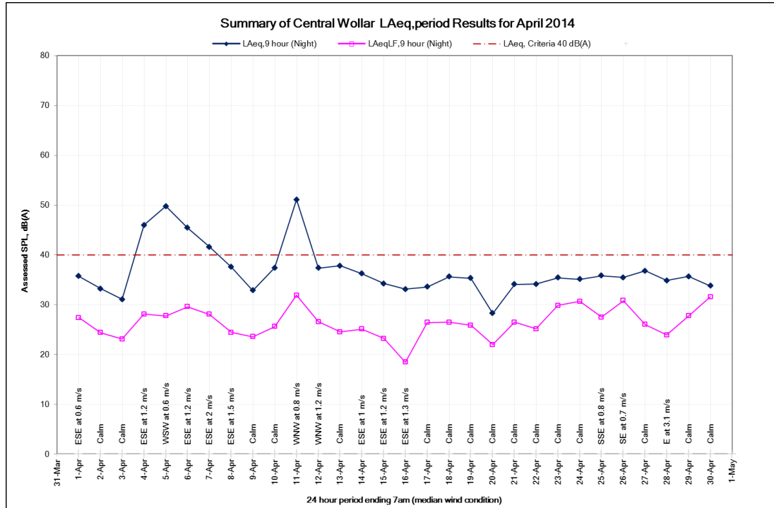
Figure 18: Night time noise levels at the Central Wollar monitoring location, April 2014
