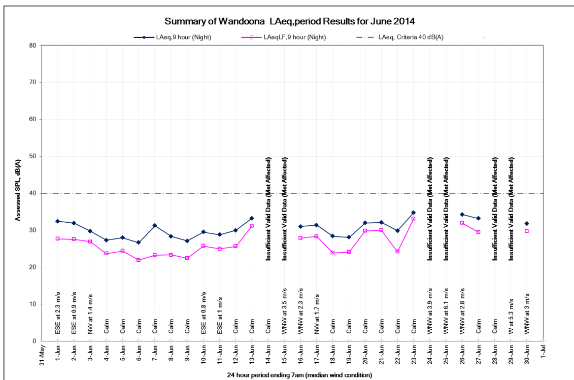
Figure 14: Night time noise levels at the Wandoona property, June 2014
