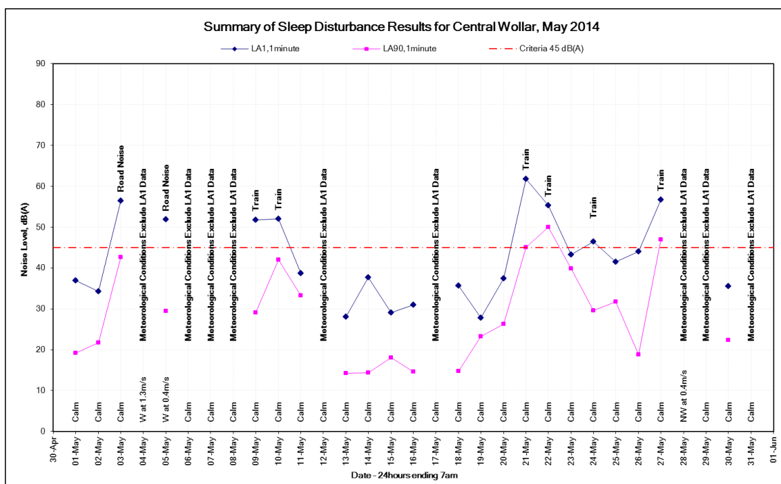
Figure 28: LA1,1minute noise levels at the Central Wollar monitoring location, May 2014
