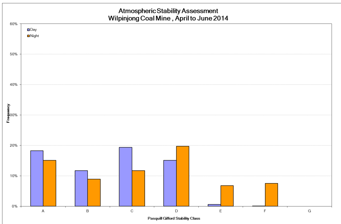
Figure 4: Assessment of temperature inversion frequency
