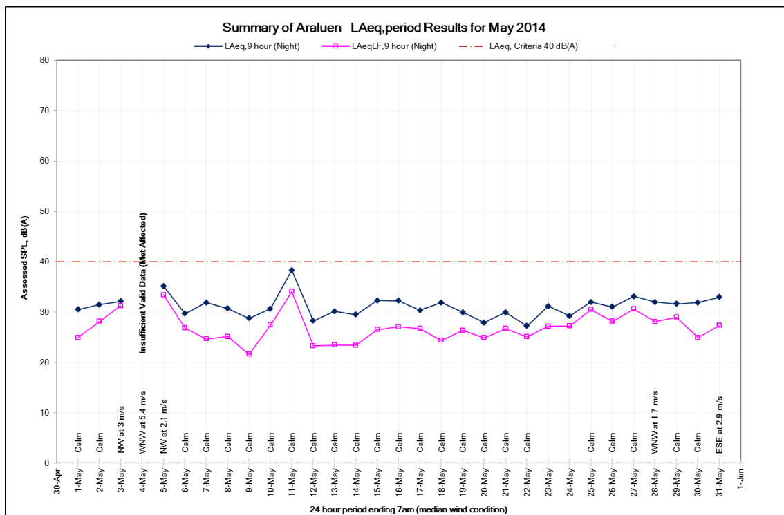
Figure 16: Night time noise levels at the Araluen monitoring location, May 2014
