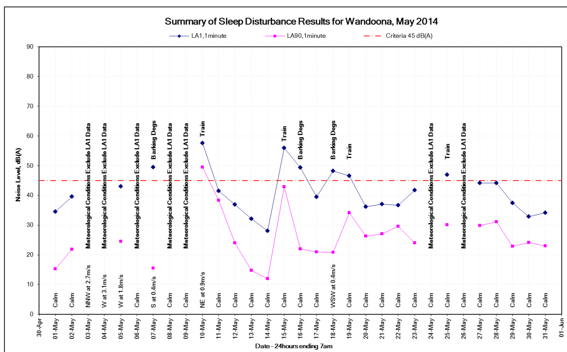
Figure 22: L_{A1,1\text{minute}} noise levels at the Wandoona monitoring location, May 2014
