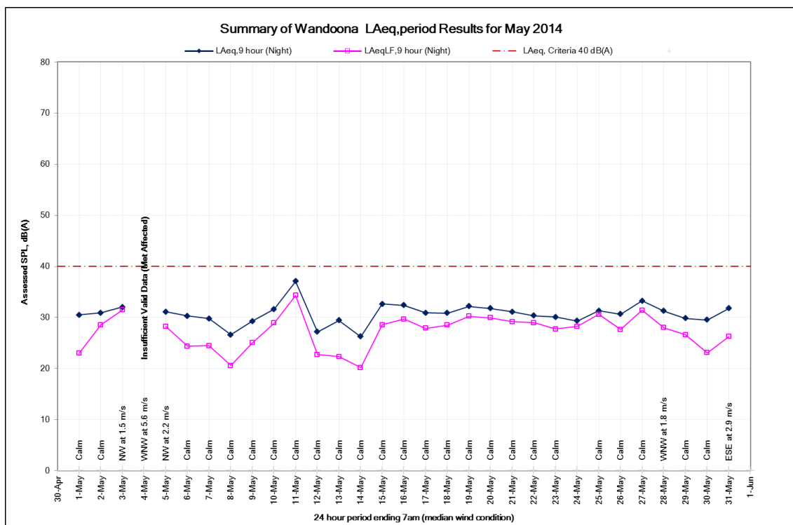
Figure 13: Night time noise levels at the Wandoona property, May 2014
