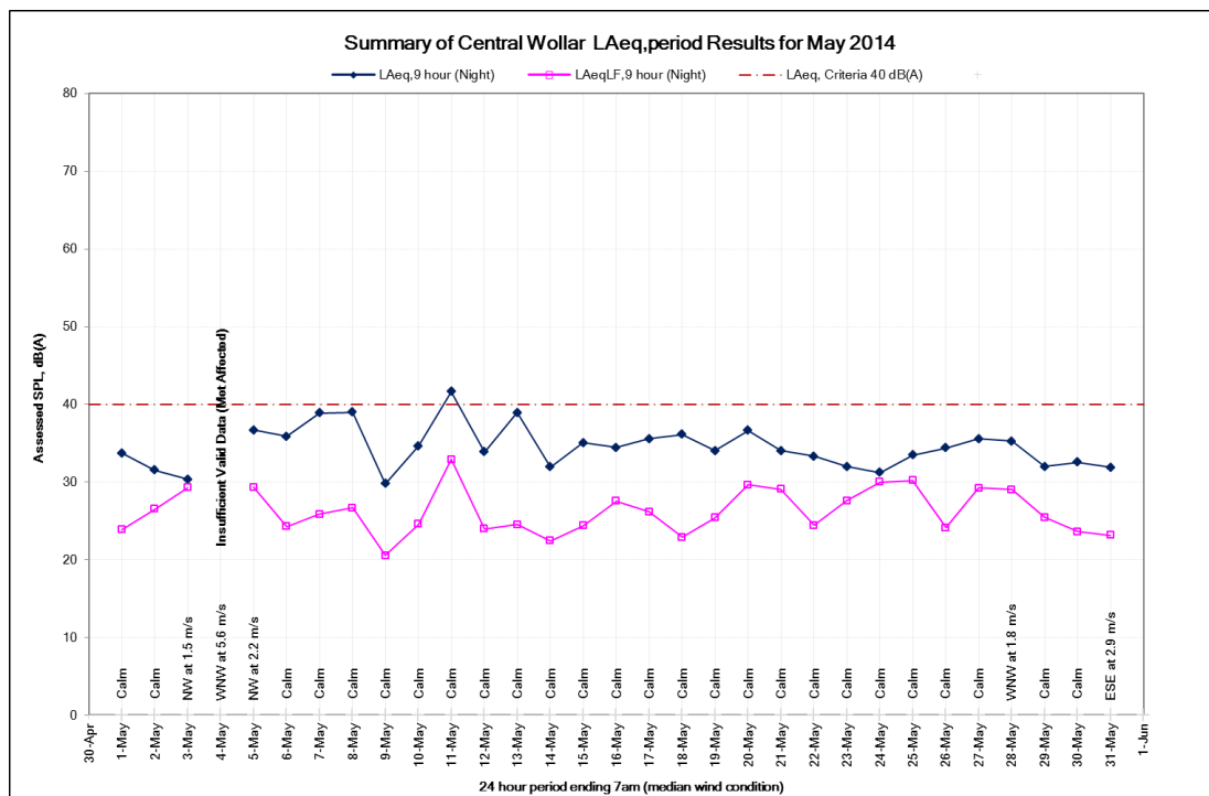
Figure 19: Night time noise levels at the Central Wollar monitoring location, May 2014
